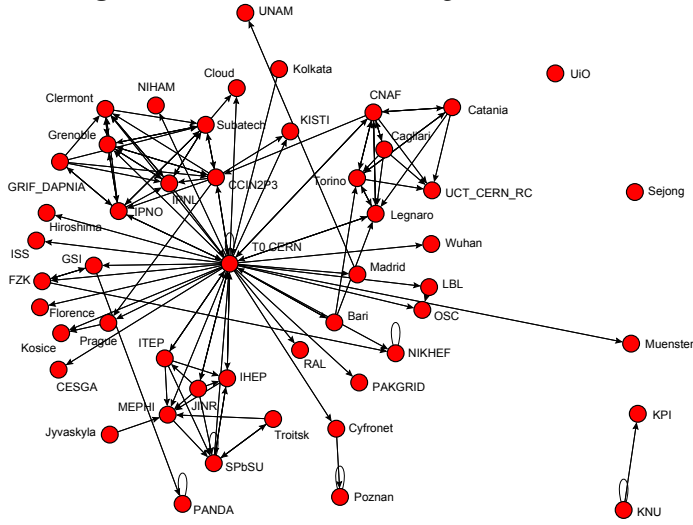
Figure 2: Email interactions among ALICE Centres
