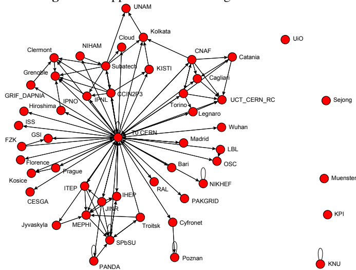
Figure 1: Support relations among ALICE Centres
